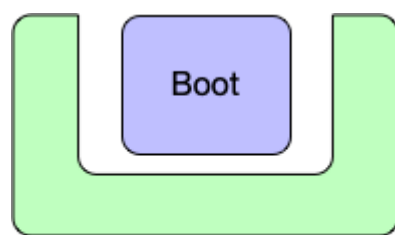
Docker container
